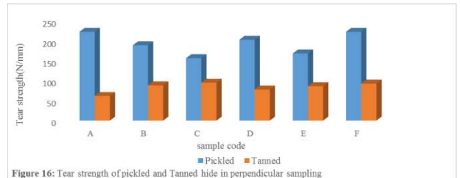
Figure 16: Tear strength of pickled and Tanned hide in perpendicular sampling
