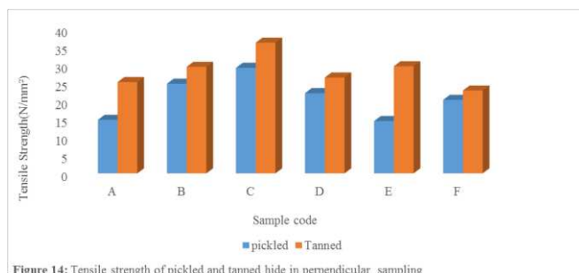
Figure 14: Tensile strength of pickled and tanned hide in perpendicular sampling
