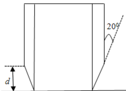
Figure 2: Schematic illustration of the shape of a press knife
