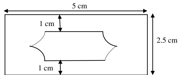
Figure 4: Schematic illustration of a standard sample for tear strength testing
