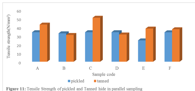
Figure 11: Tensile Strength of pickled and Tanned hide in parallel sampling
