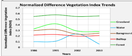
Figure 6: NDVI Trends
