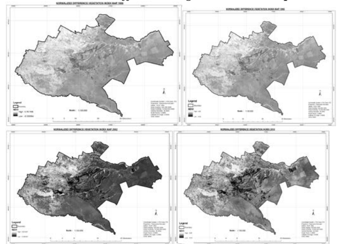
Figure 5: NDVI maps
