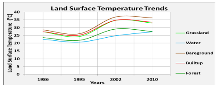
Figure 4: LST Trends
